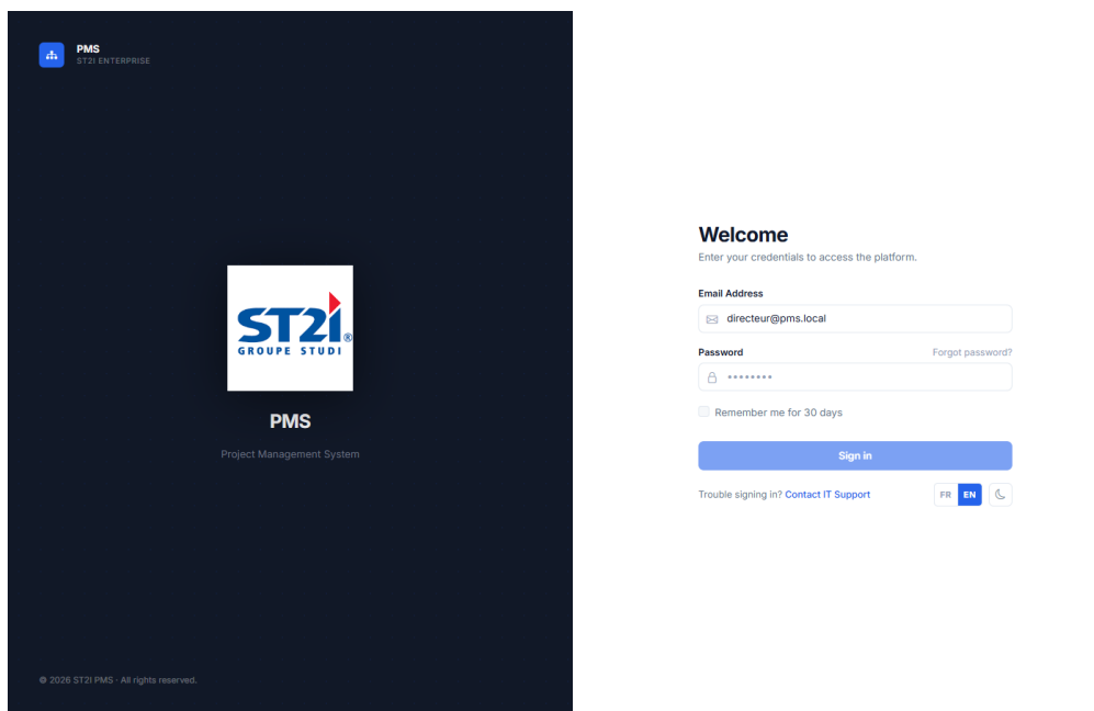
Figure 4.10: Login interface
