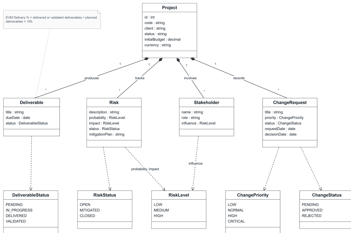
Figure 6.6: Class diagram — project governance
